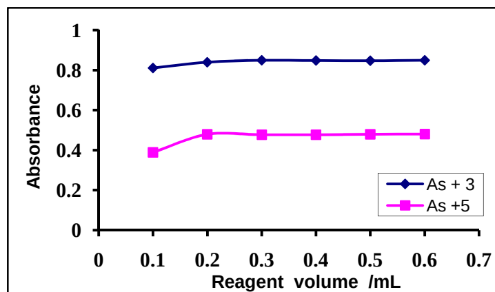
Fig. 3. Effect of concentration of 7-(6-BrBTA8HQ) / 7-(6-MBT A8HQ) on the CPE of As (III)/As (V)
