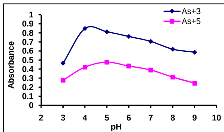
Fig. 2. Effect of pH on the formation of 7-(6-BrBTA8HQ) complex formed with As (III) and 7-(6-MBT A8HQ) complex formed with As (V).
