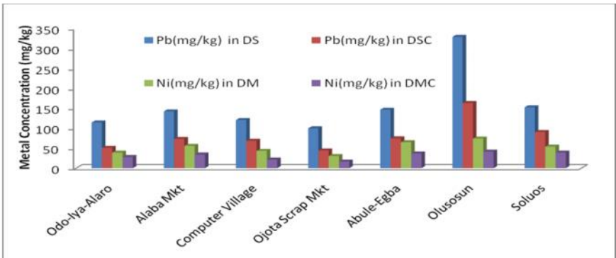
Fig.4: Comparative mean concentration of Pb and Ni (mg/kg) in dumpsites and dismantling sites with control samples. Where DS = Dumpsites, DSC = Dumpsites Control, DM = Dismantling, DMC = Dismantling Control.
