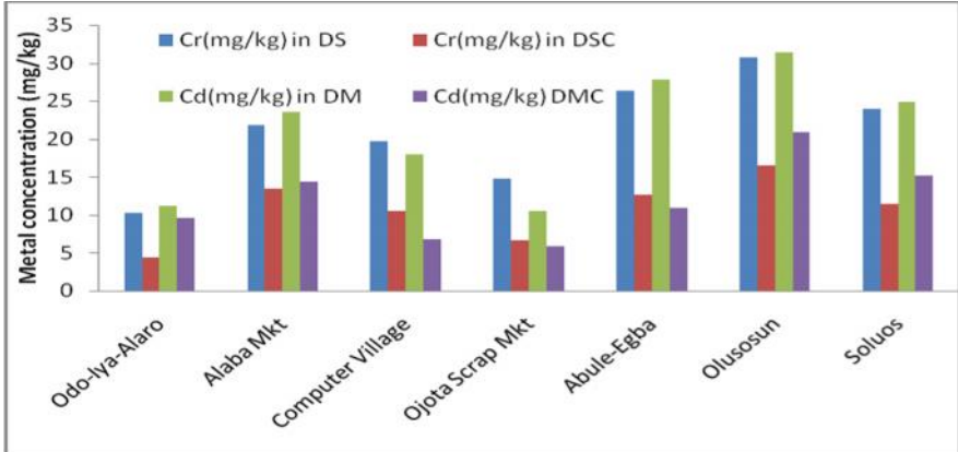
Fig.3: Comparative mean concentration of Cr and Cd (mg/kg) in dumpsites and dismantling sites with control samples. Where DS = Dumpsites, DSC = Dumpsites Control, DM = Dismantling, DMC = Dismantling Control.
