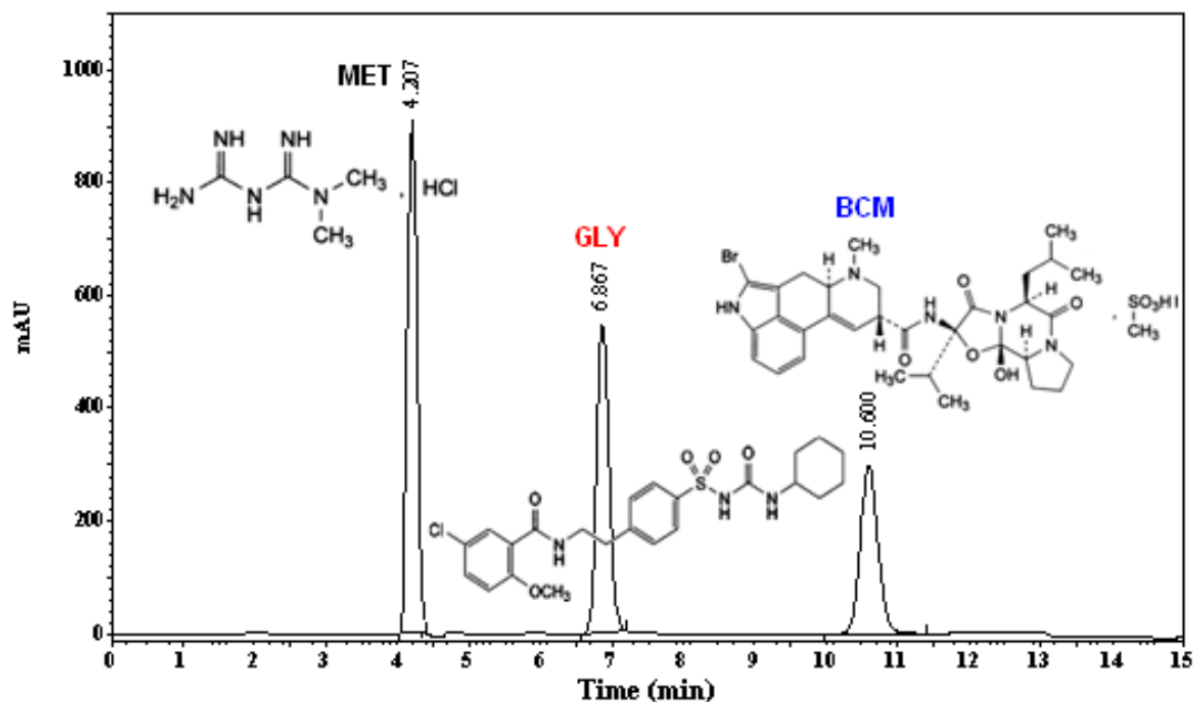
Fig. 2. A typical chromatogram of a mixture of MET (150 µg mL -1 ), GLY (150 µg mL -1 ) and BCM (200 µg mL -1 ) at retention times 4.207, 6.867 and 10.60 min, respectively. Chromatographic conditions: RP-HPLC on C 8 column; mobile phase: ammonium acetate (0.1 M - pH 5.0) /methanol (23/77, v/v); flow rate 0.7 mL min -1 and detection at 230 nm.
