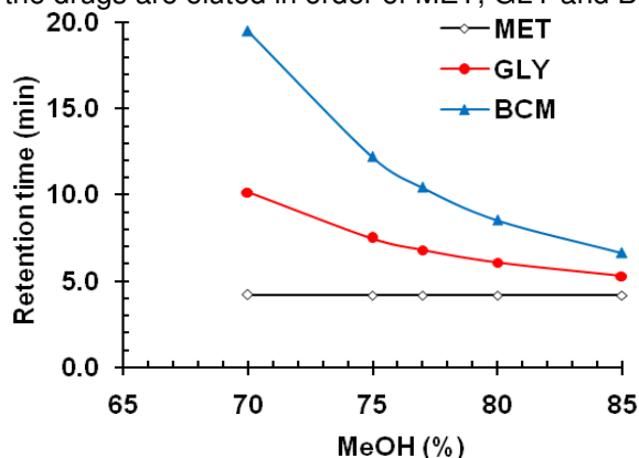
Fig. 1. plot of the retention time vs. methanol percentage in the mobile phase.
