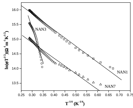
Fig.5 : The plots of \ln(\sigma T^{1/2}) versus T^{-1/4} for the films as per Greaves VRH model. Solid lines shown are the liner fits to the data.
