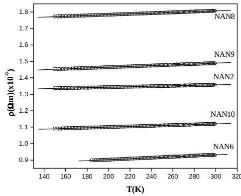
Fig.6: Plots of \rho vs T for NAN2, NAN6, NAN8, NAN9 and NAN10 films for T > 150K . The lines drawn are the linear fits to the data as per Matheissen's rule.
