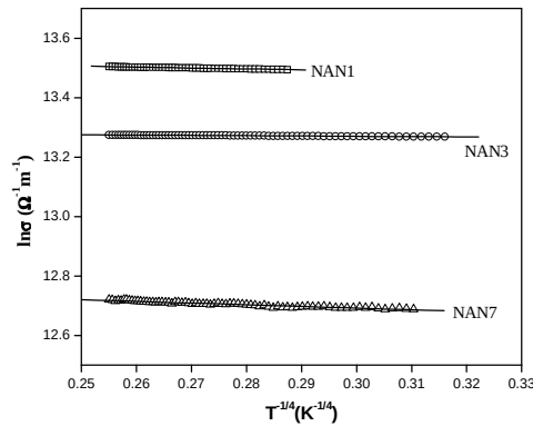
Fig. 4: Plots of \ln(\sigma) versus T^{-1/4} for NAN1, NAN3 and NAN7 films as per Mott's VRH model. Solid lines shown are the linear fits for T < (\theta_D) .
