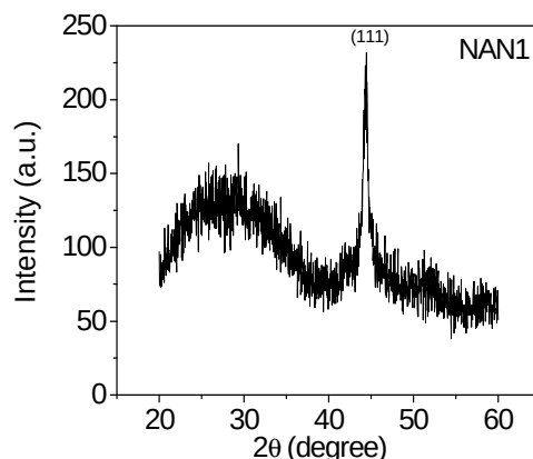
Fig.1. XRD spectra for NAN1 film.
