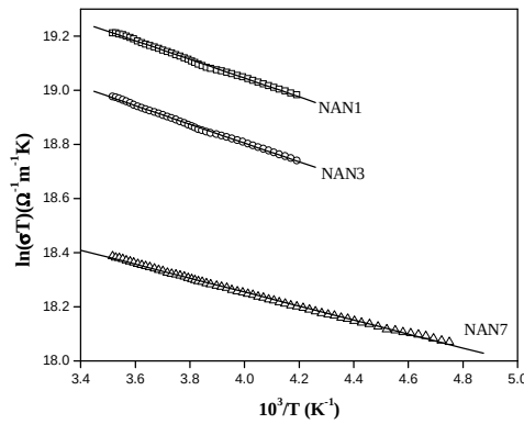
Fig. 3: The plots of \ln(\sigma T) versus (1/T) for NAN1, NAN3 and NAN7 films for T > \theta_D . Solid lines shown are the linear fits to the data
