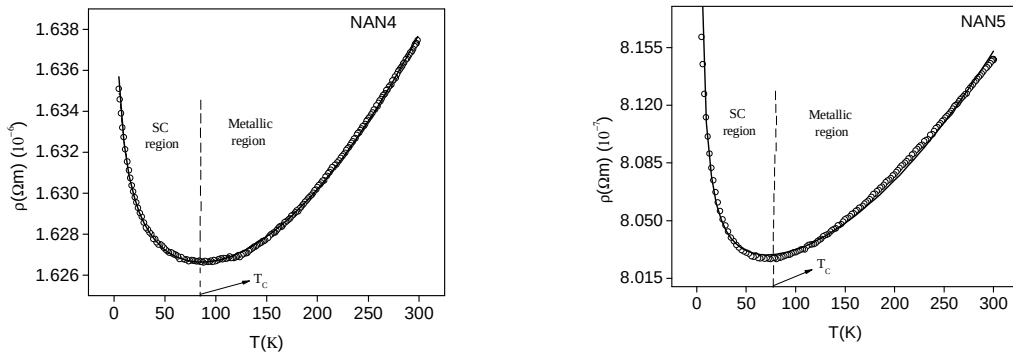
Fig.7: \rho versus T for NAN4 and NAN5 films. Solid lines are the best fits to Eq.(4).
