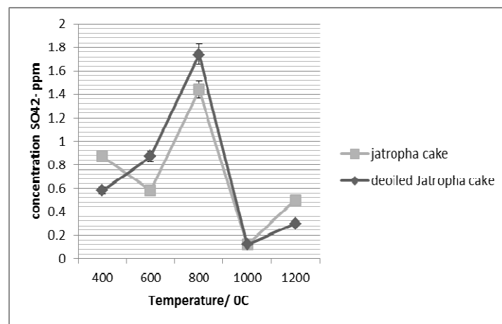
Figure 2: Effect of temperature on the amount of \text{SO}_2 produced during combustion
