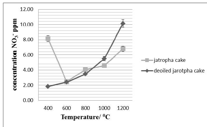
Figure 1: The effect of temperature on the amount of \text{NO}_x produced during combustion
