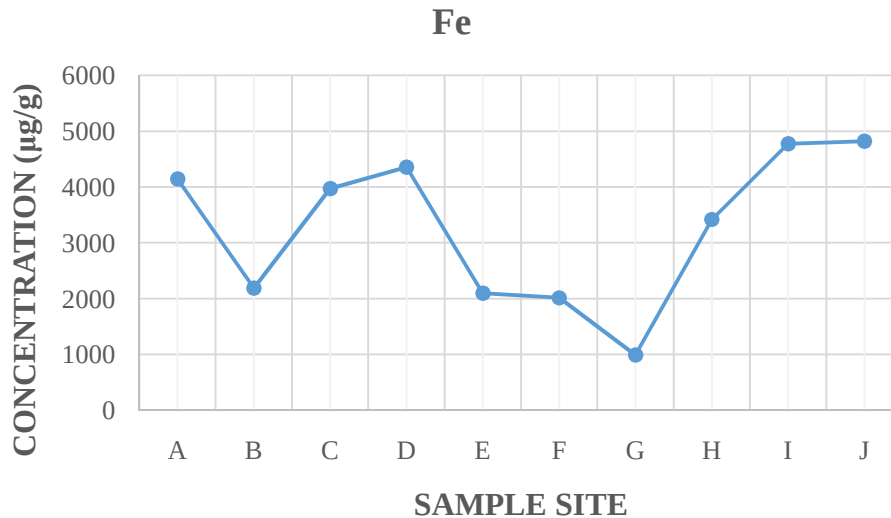
Figure 4:Concentration of Iron across the sampling site
