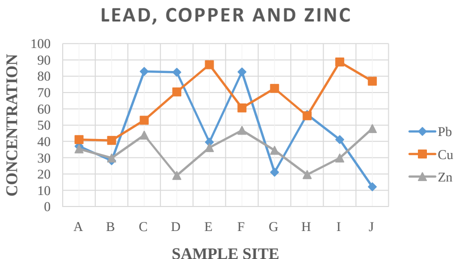
Figure1:Concentration ( \mu\text{g/g} ) of Lead, Copper and Zinc across the sampling site.
