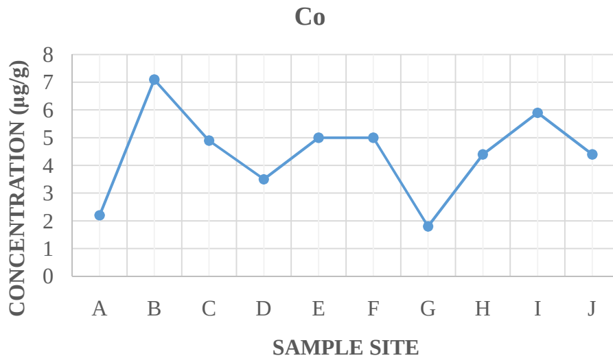
Figure2:Concentration of Cobalt across the sampling site
