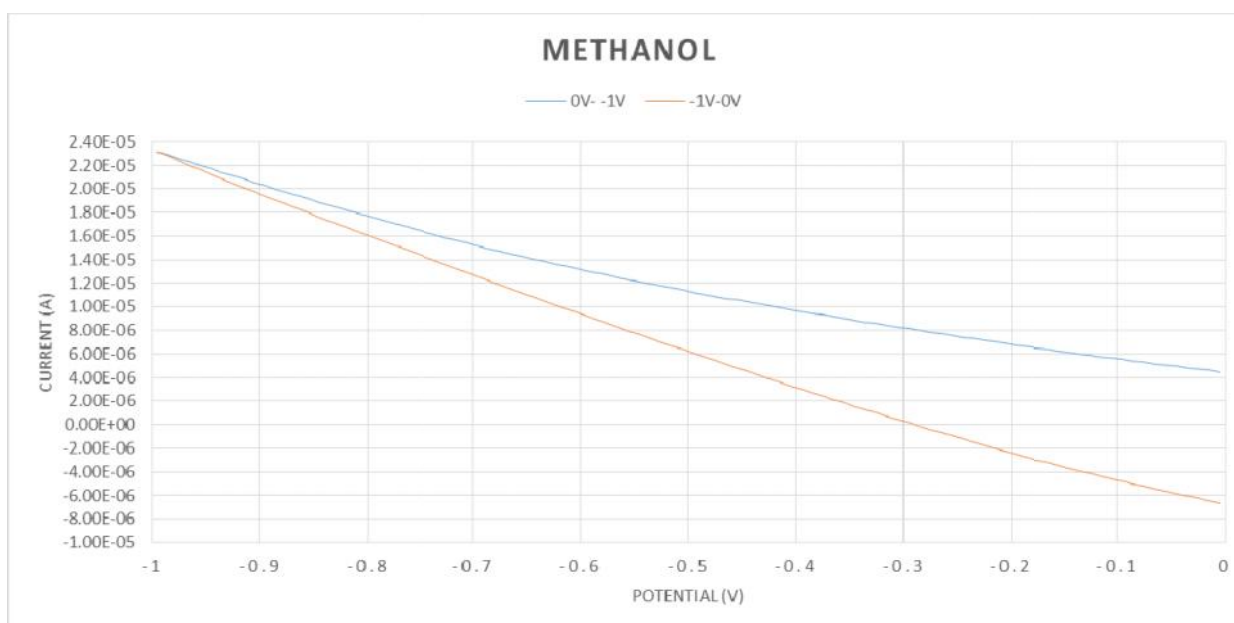
Fig. 4. Electrochemical response of methanol at the \text{TiO}_2 nanotube electrode: (a) with different anodic scanning cycles, (b) response under a cathodic scanning cycle
