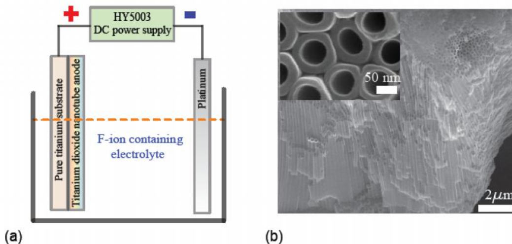
Fig. 1. Schematic of the electrochemical cell for making \text{TiO}_2 nanotubes and the image of the nanotube: (a) a sketch of the cell, (b) the image of \text{TiO}_2 nanotubes (The inset represents a high magnification image confirming the formation of the nanotubes)
