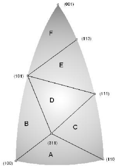
Fig. 2. Etching rate model regions used in our 3D simulations.
