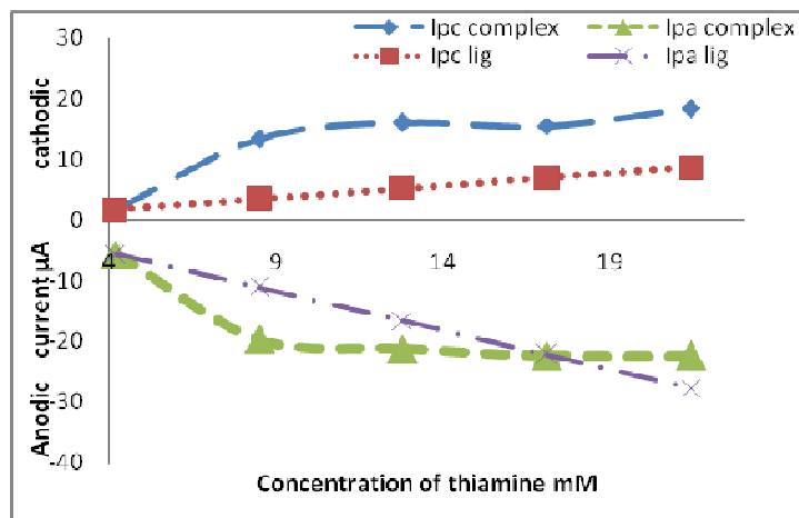
Fig. 7. Plot between I_{pc} versus variable concentration of thiamine HCl than ferrous ion complexes solution in acidify pH at 100mV/s scan rate.
