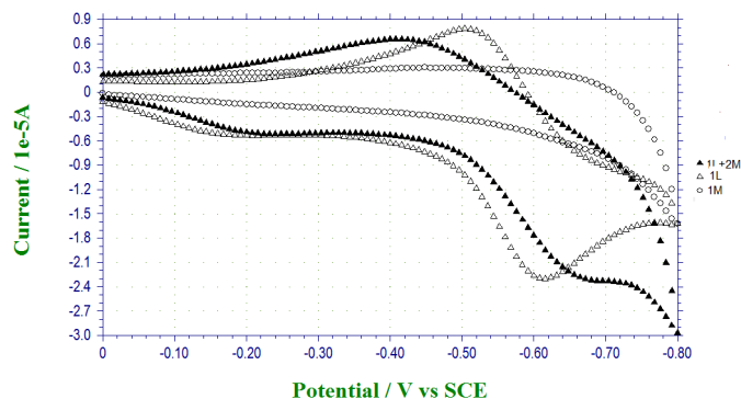
Fig. 3. Voltammogram of ferrous, thiamine and (1L:2M) complex solution at 100 mV/s.
