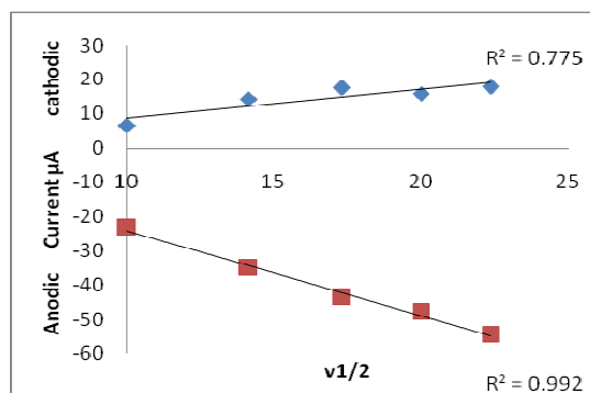
Fig. 5. Plot of v_{1/2} and I_{pa} or I_{pc} of 1:2 mole ratio complex.
