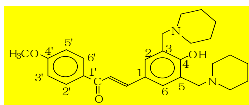
Figure 4: 4-hydroxy-4'-methoxy-3,5-bis-pyrrolidinomethylchalcone ( 3 )
