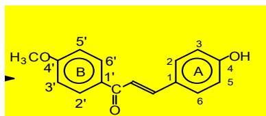
Figure 1: 4-hydroxy-4'-methoxychalcone (1)
