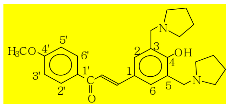
Figure 3: 4-hydroxy-4'-methoxy-3,5-bis-pyrrolidinomethylchalcone ( 3 )
