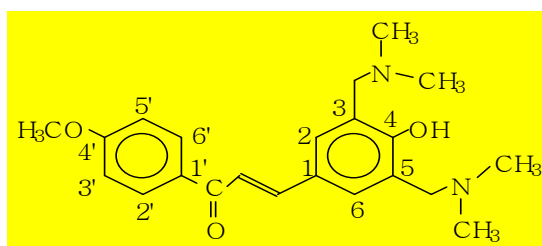
Figure 2: 4-hydroxy-4'-methoxy-3,5-bis-dimethylaminomethylchalcone(2)
