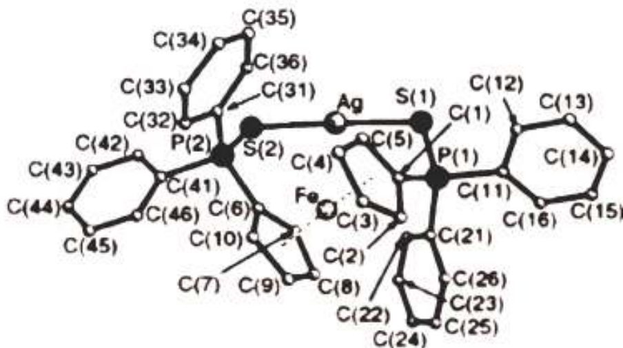
Figure 1. Structure of [\text{Fe}(\text{dtpc})\text{Ag}]^+ [5]
