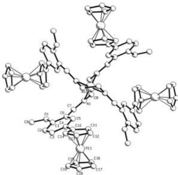
463 Figure 4. Structure of [(cp)_2Fe_2(eimp)_2]_2Ag [17]
