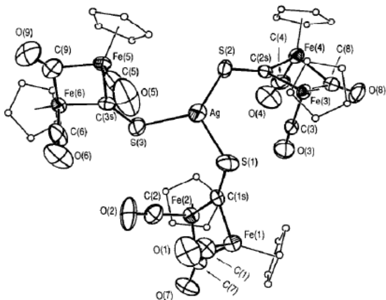
465 Figure 5. Structure of [(cp)_2(CO)_3Fe_2(CS)]_3Ag [21]
