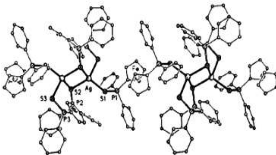
Figure 7. Structure of [\{\text{CH}_2(\text{Ph}_2\text{PS})_2\text{Ag}\}_2(\text{dptdf})_2]_n^{2+} [28]
