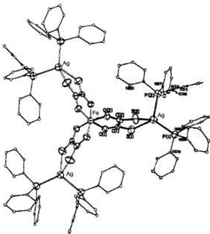
Figure 3. Structure of [\text{Fe}(\text{O}_2\text{C}_2\text{S}_2)_3\{\text{Ag}(\text{PPh}_3)_2\}_3] [16]
