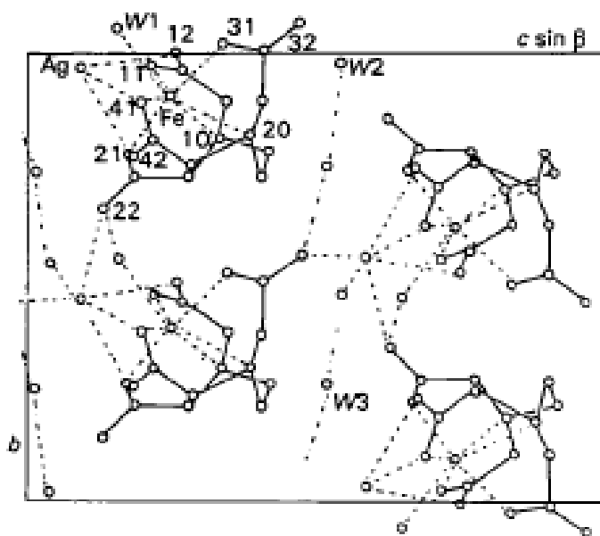
Figure 6. Structure of [(\text{H}_2\text{O})\text{Fe}(\text{edta})\text{Ag}(\text{H}_2\text{O})_2] [26]
