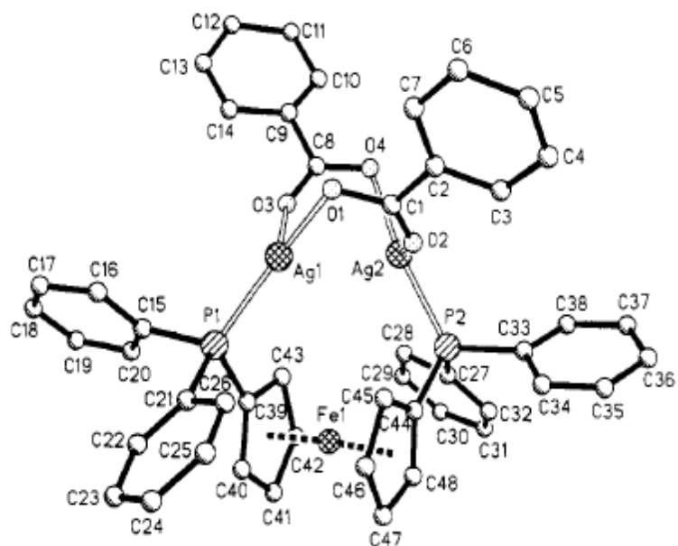
Figure 2. Structure of [\text{Fe}(\text{C}_5\text{H}_4\text{PPh}_2)_2\text{Ag}_2(\text{bz})_2] [12]
