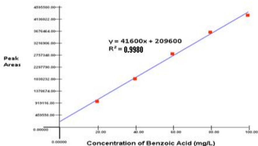
Fig.2. Calibration curve for standard Benzoic Acid
