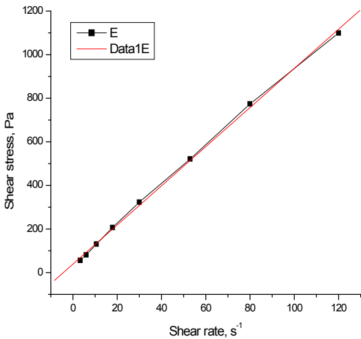
Fig. 4. Rheograms of sunflower oil at 70 °C
