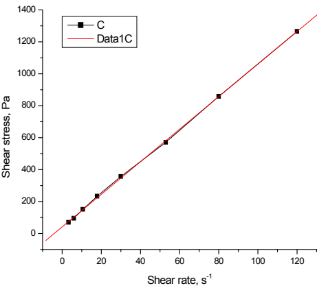
Fig. 2. Rheograms of sunflower oil at 50 °C
