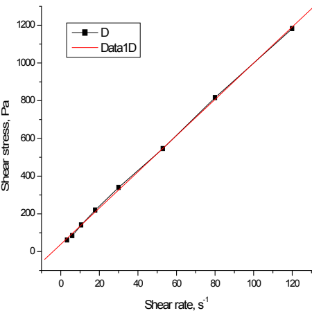
Fig. 3. Rheograms of sunflower oil at 60 °C
