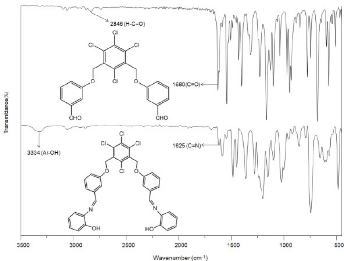
Fig. 3. Comparative FT-IR spectra of dialdehyde and di-imine
