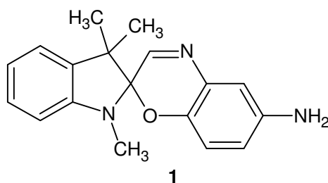
Structure of Indolino spirobenzoxazine
