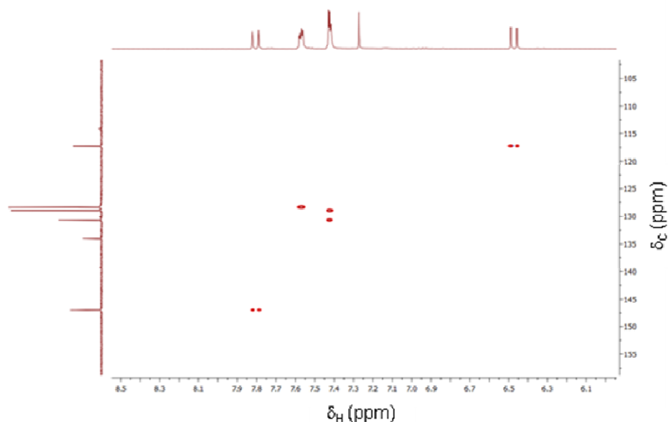
Figure 3 HSQC spectrum of \text{H}_{71} fraction
