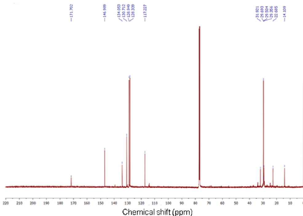
Figure 1 ^{13}\text{C} NMR spectrum of \text{H}_{71} fraction (125 MHz, \text{CDCl}_3 )
