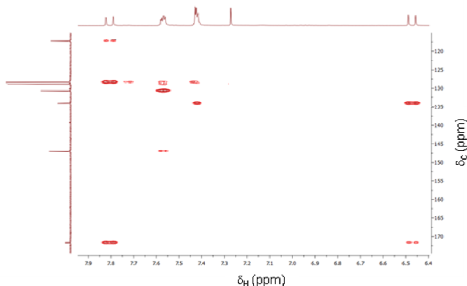
Figure 4 HMBC spectrum of H 71 fraction
