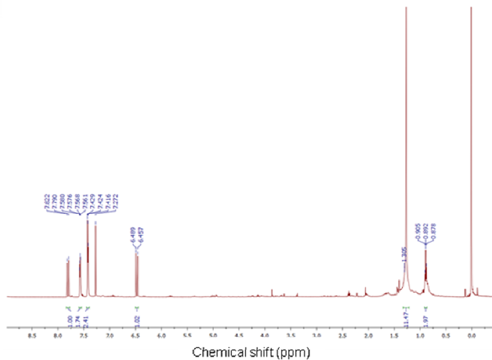
Figure 2 ^1\text{H} NMR spectrum of \text{H}_{71} fraction (500 MHz, \text{CDCl}_3 )
