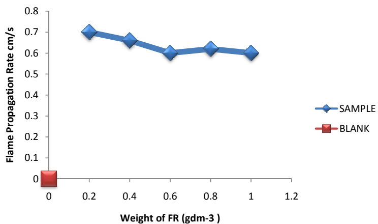
Figure 3: Effect of Concentration on Flame Propagation Rate
