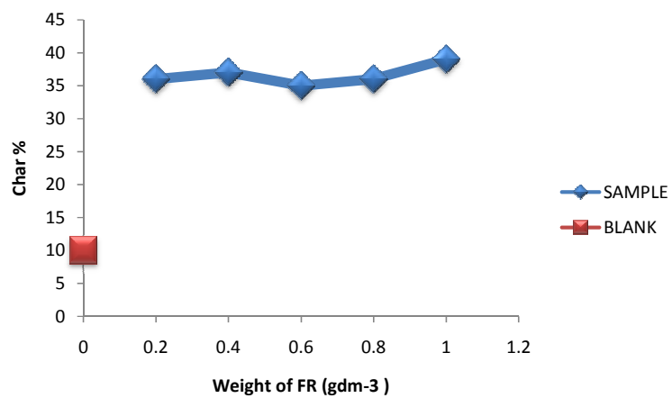
Figure 5: Effect of Concentration on Char %
