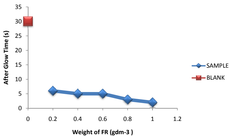
Figure 4: Effect of Concentration on After Glow Time
