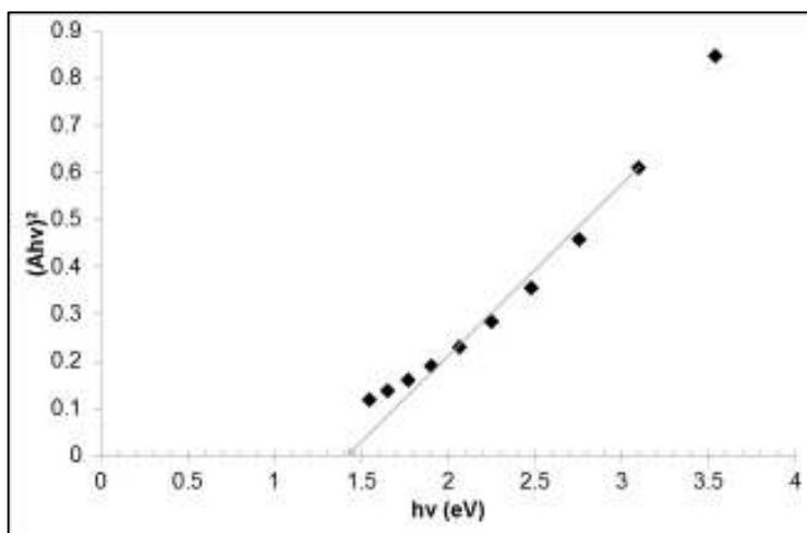
Fig. 4. Plot of (Ah\nu)^2 versus h\nu for the \text{Ni}_3\text{Pb}_2\text{S}_2 thin films.
