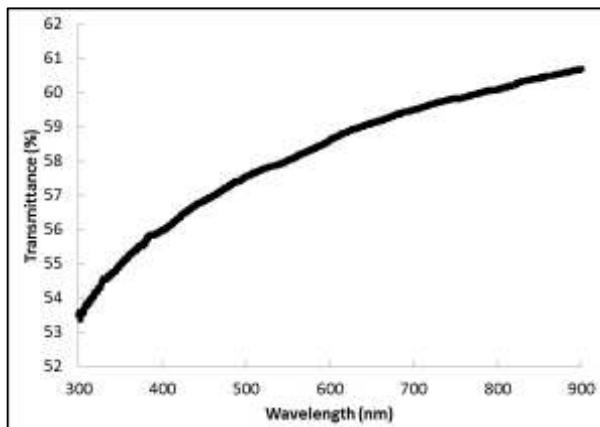
Fig. 2. Transmittance spectrum of \text{Ni}_3\text{Pb}_2\text{S}_2 thin films
