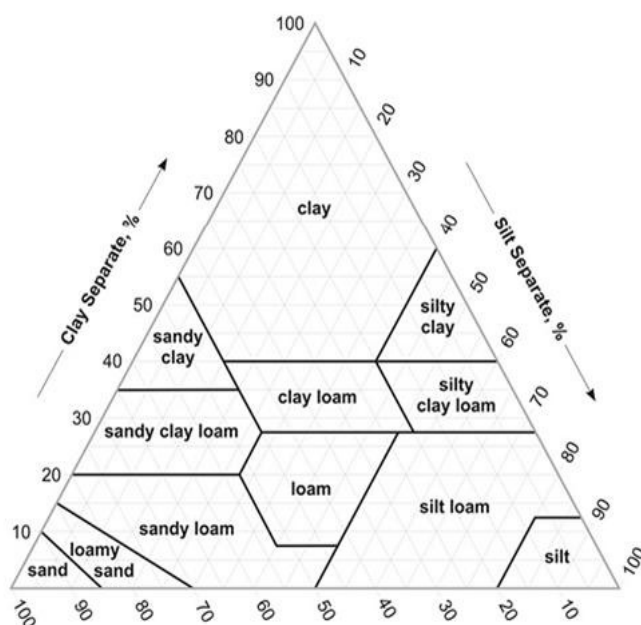
Fig. 2. Triangular diagram of textural classes of soil
