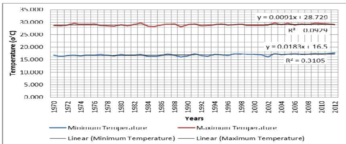
Figure 1: Minimum and maximum temperature trends from 1970 to 2012. Source: TMA-Dodoma station (2013).
