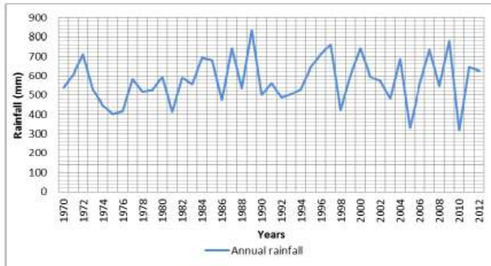
Figure 4: Annual rainfall variability from 1970 to 2012. Source: TMA-Dodoma station (2013).
