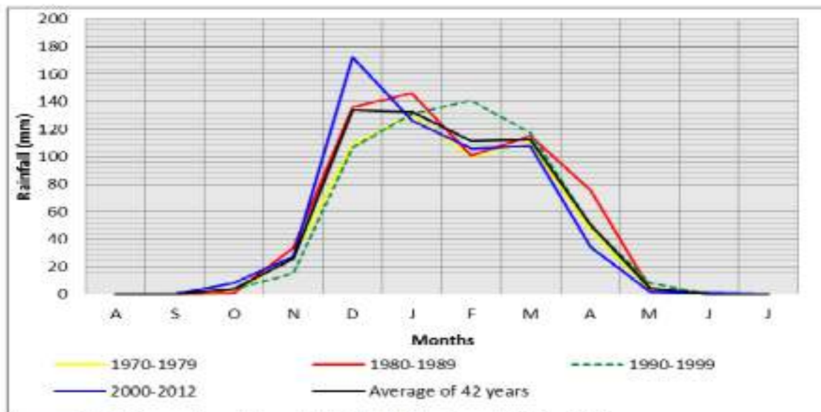
Figure 3: Variations of monthly rainfall distribution from 1970 to 2012. Source: TMA-Dodoma station (2013).
