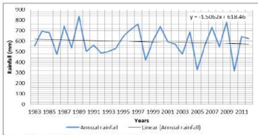
Figure 6: Annual rainfall trend from 1983 to 2012.
