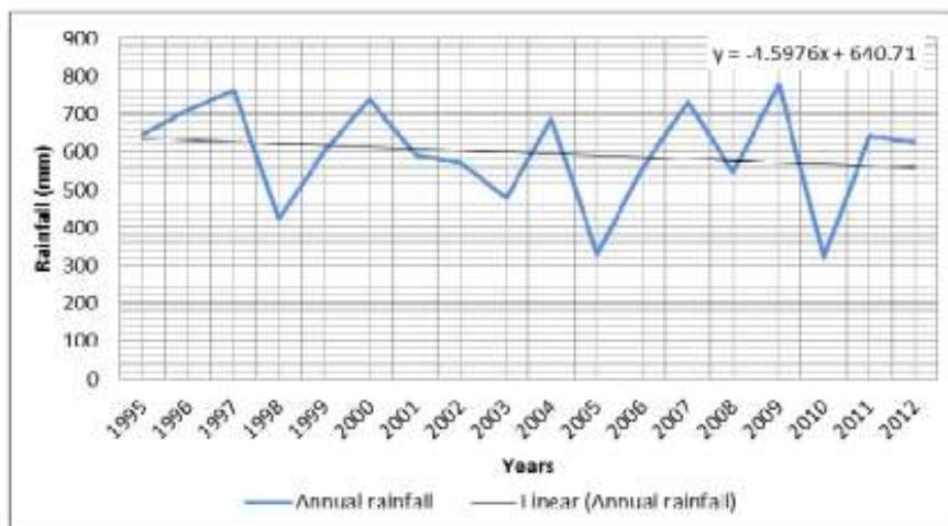
Figure 5: Annual rainfall trend from 1995 to 2012. Source: TMA-Dodoma station (2013).
