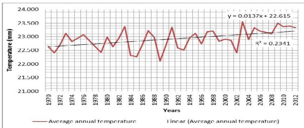
Figure 2: Average annual temperature trend from 1970 to 2012. Source: TMA-Dodoma station (2013).
