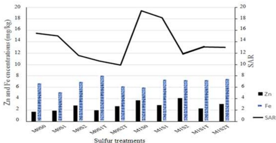
Figure 2: Interactive effects organic matter and sulfur on SAR and Fe and Zn concentrations
