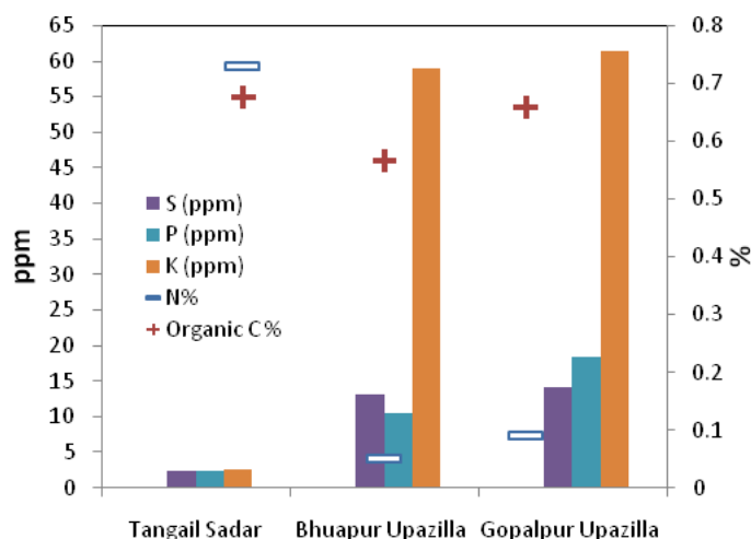
Fig. 4. Macronutrient contents in study area
