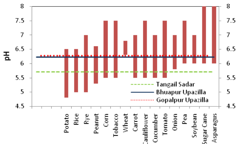
Fig. 3. The pH of the study areas and suitable range for various crops cultivation
