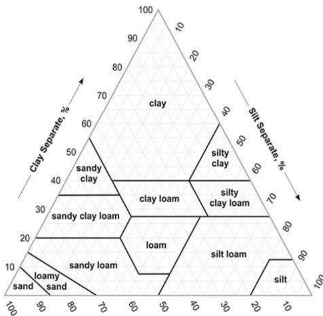
128 129 130 Fig. 2. Triangular diagram of textural classes of soil 131
