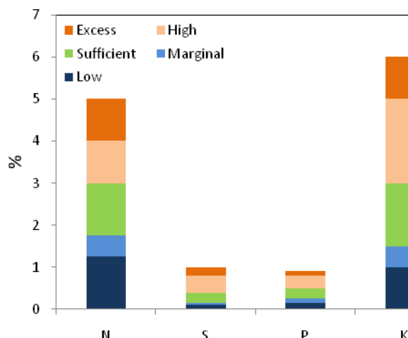
Fig. 5. The recommended level of nutrients for a variety of plants
