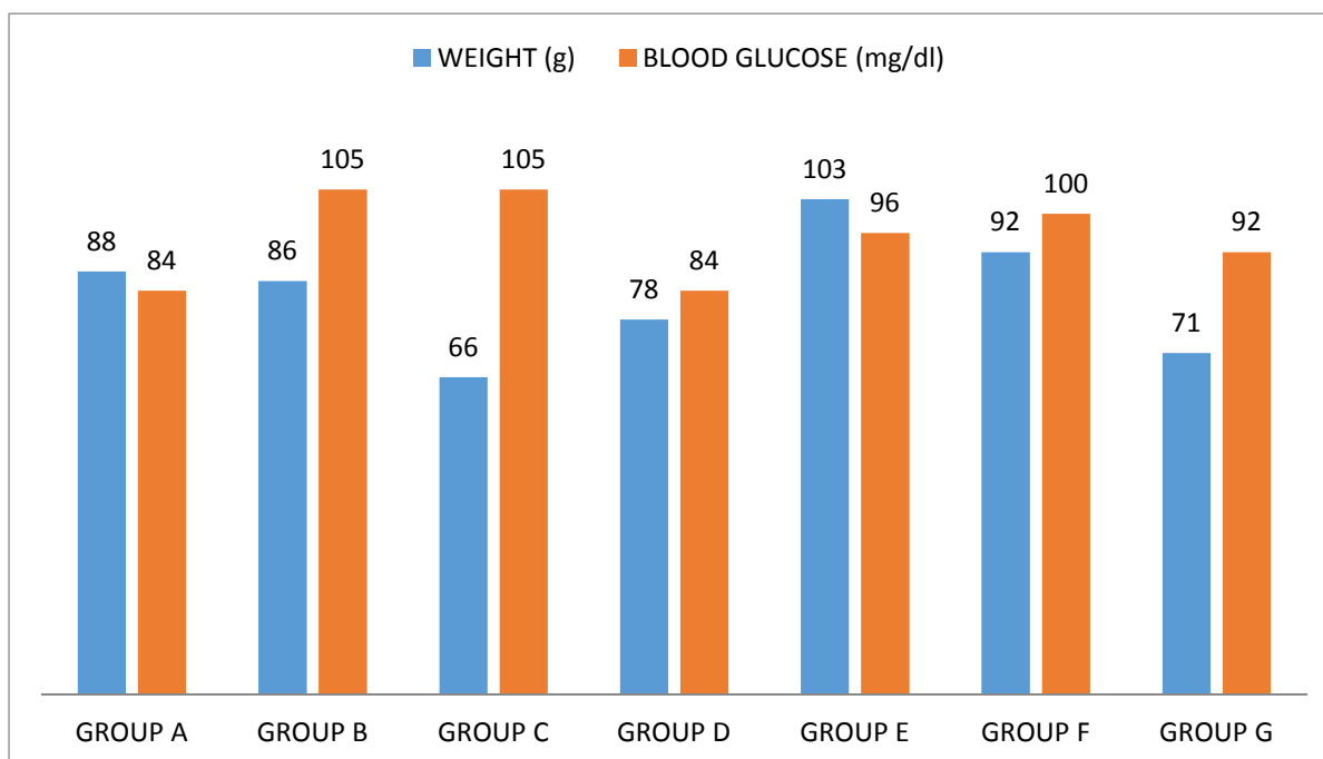
Figure 1: Bar chart showing weight and blood glucose at the third week; blood sugar levels were altered in the treated groups relative to the control. Animal Groups include A- G: Group A is the Control [fed ad libitum ]; Groups B, C, D, E, F and G were exposed to cadmium sulphate toxicity [2.5 mg/kg]. Group B animals were untreated; Group C was treated with daily oral administration of 100 mg/kg vitamin C and Group D, 30 mg/kg vitamin E; Groups E was treated with 4 mg/kg of Moringa seed oil and Group F, 4 mg/kg of Cashew nut oil - orally and daily while Group G received daily oral administration of 2 mg/kg of Moringa oleifera oil and 2 mg/kg of Cashew nut oil [combined]. The blood sugar levels were altered in the treated groups relative to the control; it was highest in the untreated Group B and vitamin treated Group C; it was lowered in every other group relative to the control. Weights were taken for reference,
