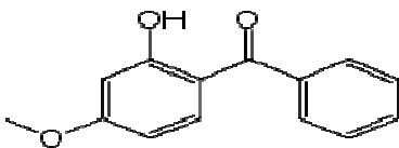
Fig. 1. Chemical structure of Benzophenone-3
