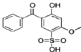
Fig. 2. Chemical structure of Benzophenone 4
