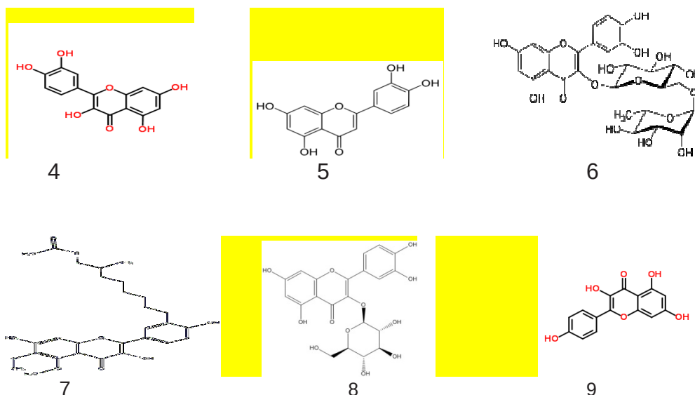
Fig 2: Chemical structures of flavonoids of S. kunthianum
