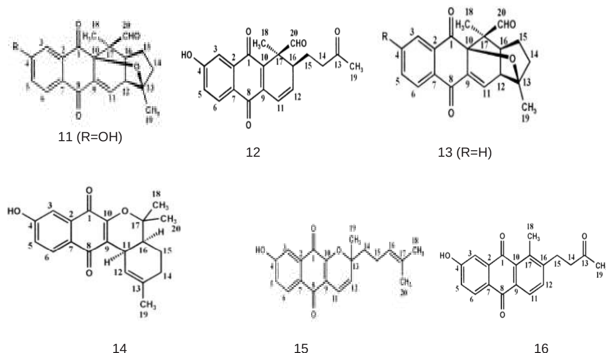
Fig 4: Chemical structures of quinones of S. kunthianum
