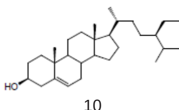
Fig 4: Chemical structure of sterol S. kunthianum
