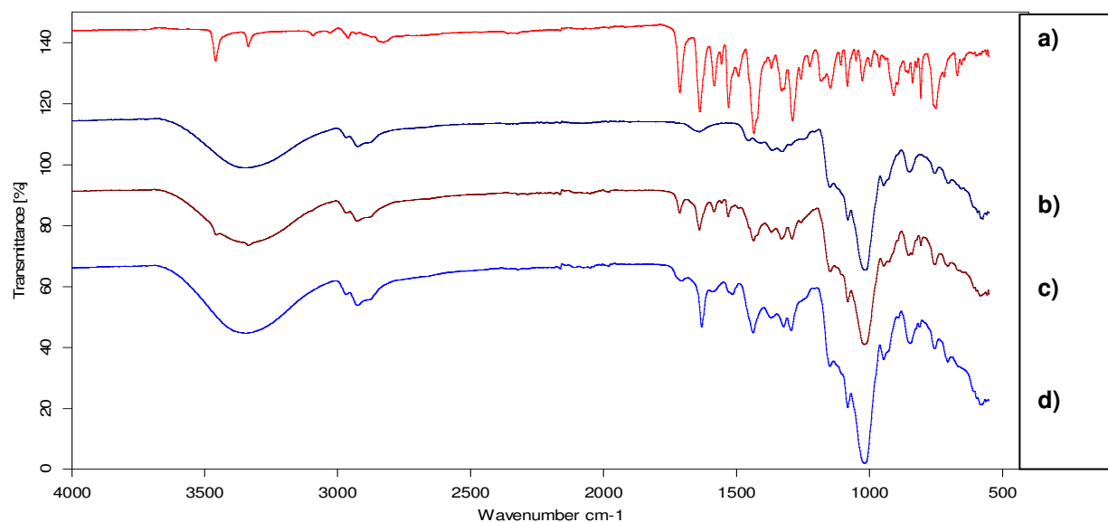
Figure (4): FT-IR spectra of a) sparfloracin, b) HP- \beta -CyD, c) physical mixture and d) spray dried complex
