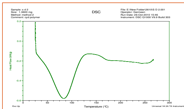
Figure (4): DSC thermograms of A) HP-β-CyD, B) sparfloxacin, C) physical mixture and D) Spray dried complex
