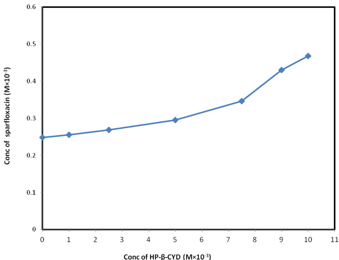
Figure (3): Phase solubility diagram of sparfloxacin
