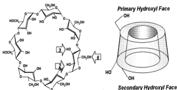
Figure (2): The structure of HP-β-CyD
