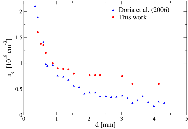
Figure 9: The free electron density distribution of Li II versus normal distance from the sample surface d . Comparison is made with the estimation values in Ref. [Doria et al. (2006)] at 60 ns delay time.
