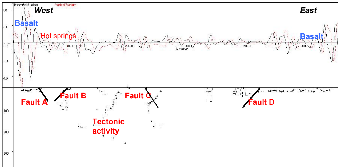
Figure 11 a Geologic map of the magnetic survey area. (b) Processed ground magnetic data with 2D Euler solutions obtained along traverse one with inclination and declination angles of -26.2^\circ and 0.03^\circ respectively. Plus (+) signs are Euler solutions for 1.0 structural index.
