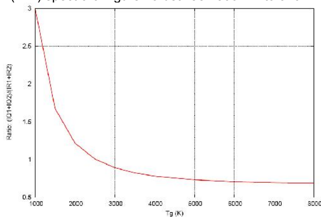
Fig. 12. Variation versus the gas temperature of the ratio R_{IQIR} of the intensities of Q1 and Q2 branches over the intensities of R1 and R2 branches in the case of synthetic spectra of OH(A-X) emissions
