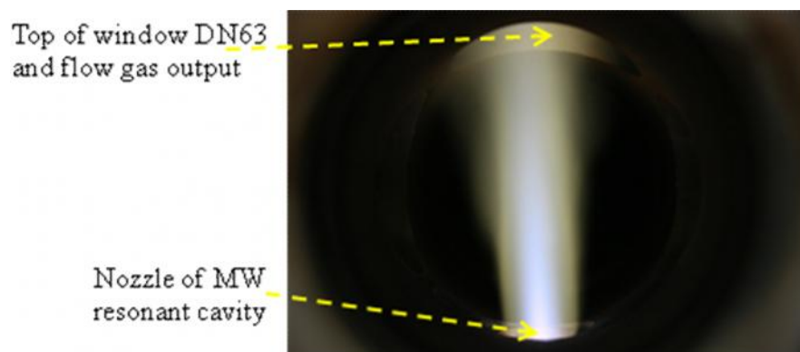
Fig. 2. Air plasma column inside the cell for P_{MW} = 1kW , Air gas flow=12 l/min and pressure=600 mbar.
