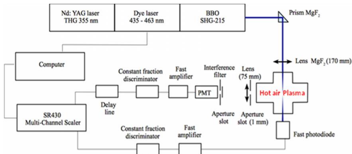
Fig. 3. Schematic view of the experimental setup for TALIF diagnostics used for measurement of Oxygen atom.
