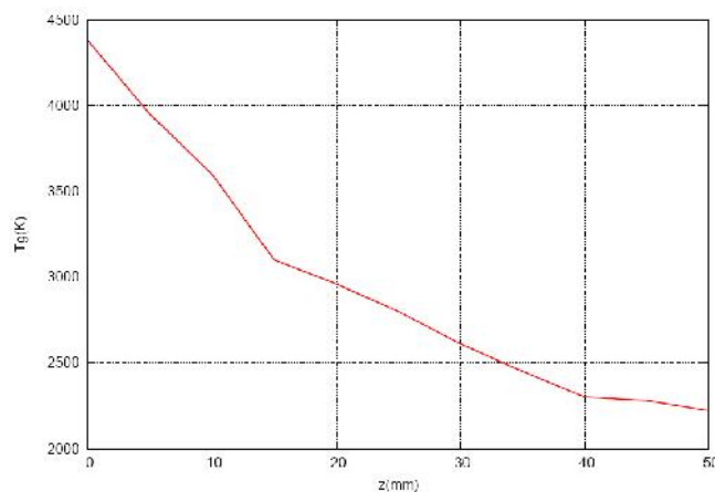
Fig. 14a. Measured gas temperature along the axis of the air plasma column in the case of P_{MW}=1 kW, Pressure=600 mbar, inlet gas composition=Air+3% H_2 , and Gas flow=12 l/min.
