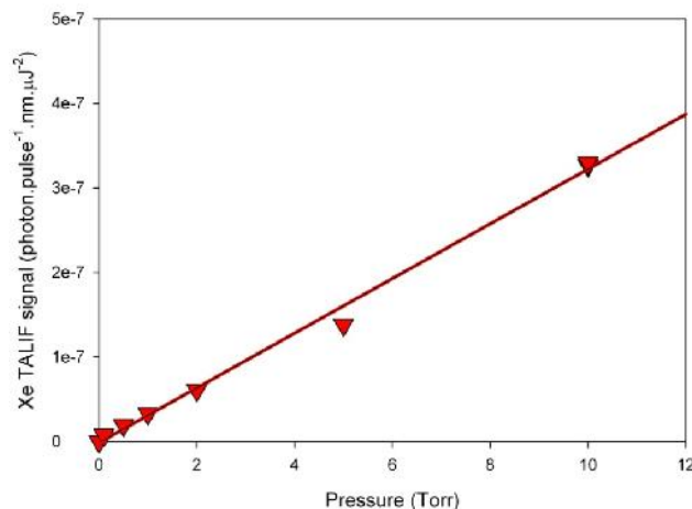
Fig. 10. Integrated and normalized xenon TALIF signal as a function of the xenon pressure. Fluorescence recorded through an interference filter centred at 830 nm (Bandwidth = 10 nm).
