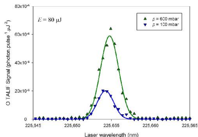
Fig. 7. Two-photon line profiles of the O(2p^4 \ ^3P_{0,1,2} \rightarrow 3p^3 \ ^3P_J) transitions obtained in the plasma jet at two different pressures. (Air flow= 11.64 L/min, H_2 flow= 0.36 L/min, P_{MW} = 1 kW) .
