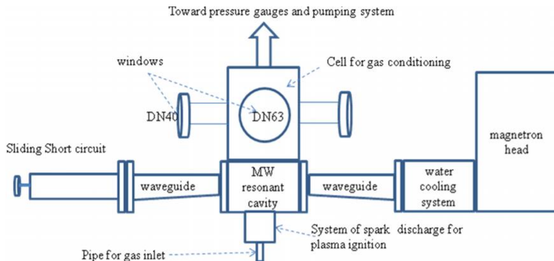
Fig. 1. Schematic view of the experimental setup including the microwave resonant cavity with the cell of gas conditioning and the 2.45GHz microwave generator with a magnetron head and a power supply not shown in this scheme.
