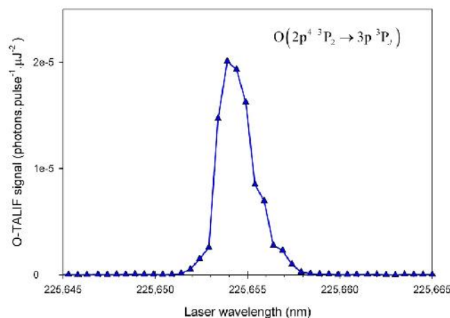
Fig. 6. Two-photon excitation line profiles of the O(2p^4 \ ^3P_{0,1,2} \rightarrow 3p^3 \ ^3P_J) transitions obtained in the plasma column in the center of the cell at 600 mbar, Air flow= 11.64 L/min, H_2 flow= 0.36 L/min, P_{MW} = 1 kW
