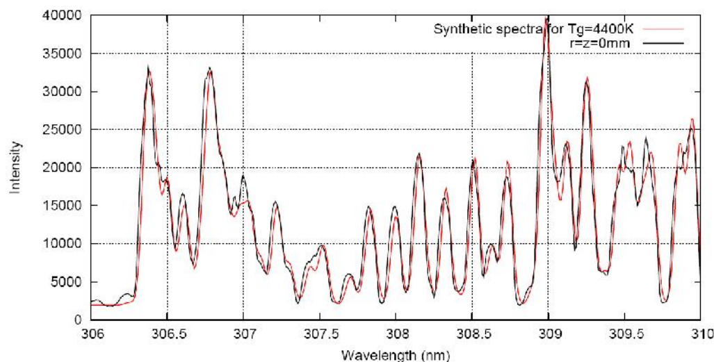
Fig. 13. Comparison between experimental spectrum and calculated one for T_g=4400K at the position of plasma column: r=0 , z=0 (in the center of plasma column and near the nozzle) in the case of P_{MW}=1 kW, Pressure=600 mbar, inlet gas composition=Air+3% H_2 , and Gas flow=12 l/min.
