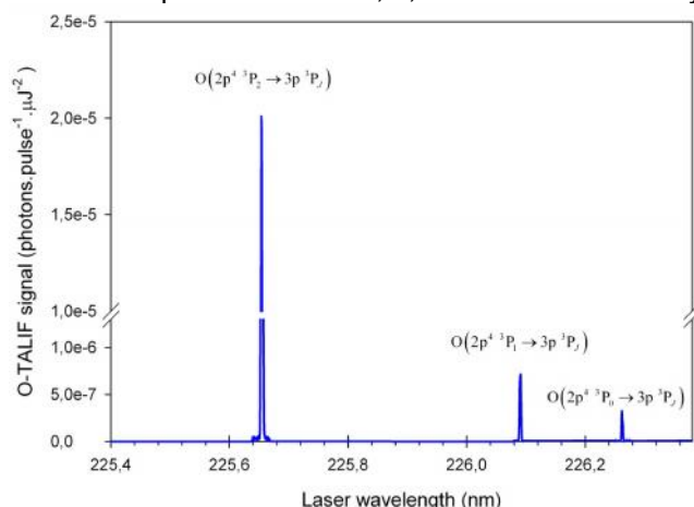
Fig. 5. Two-photon excitation spectrum of atomic oxygen (emission wavelength: 845 nm) recorded in the plasma column in the center of the cell at 600 mbar, Air flow= 11.64 L/min, \text{H}_2 flow= 0.36 L/min, P_{\text{MW}} = 1 \text{ kW} .
