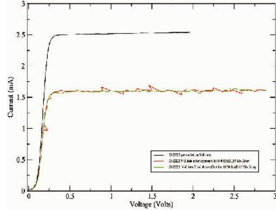
Figure 6: Effect of cumulative dose of 15 MV –rays to produce random noise.
