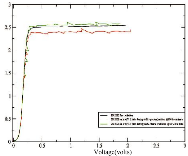
Figure 4: Effect of dose rate of 6 MV -rays to produce random noise.
