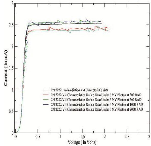
V-I Characteristics of 2N 2222 under 6MV photon at doses of 300,500,1000,2000 RADs
