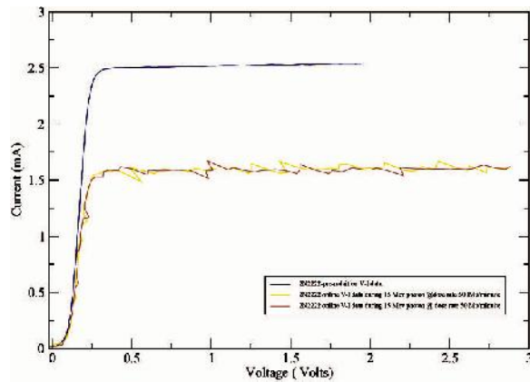
Figure 5: Effect of dose rate of 15 MV -rays to produce random noise.
