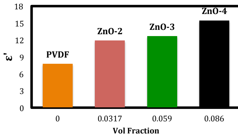
Fig 3. Dielectric constants for composites as a function of volume percent of ZnO
