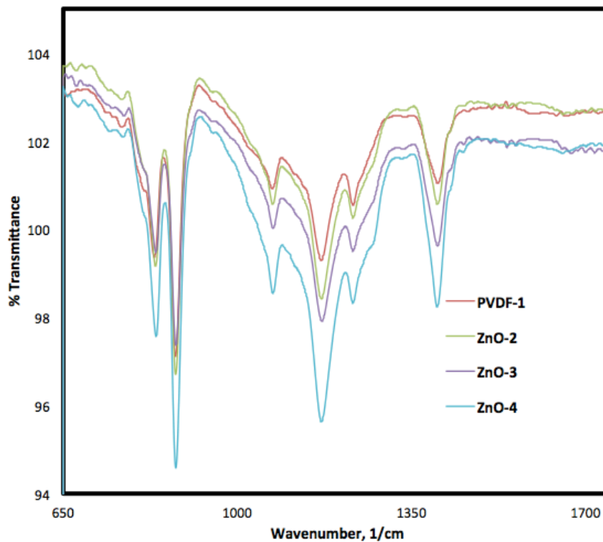
Fig 4. FTIR spectra of PVDF and PVDF/ZnO nanocomposites
