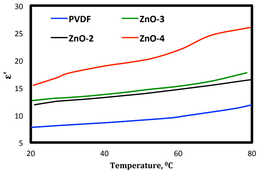
Fig 2. Dielectric constant vs. temperature for various concentrations of ZnO
