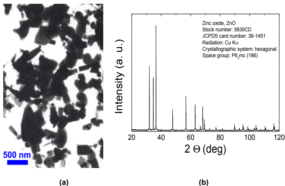
Fig 1. (a) TEM image of ZnO NP, (b) XRD spectra of ZnO NP
