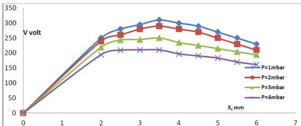
Figure (4): axial potential distribution in the absence of the magnetic field at edge and at constant current ( I=10\text{mA} ) for Helium
