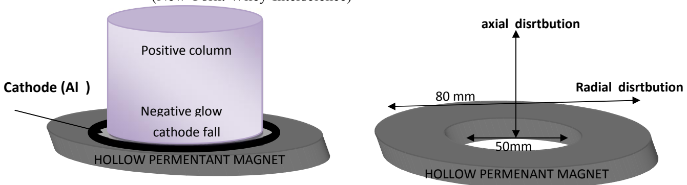
Figure (1.a,b): (a) A schematic diagram of the plasma cell , (b) the radial and axial distribution for the magnetic field strengths
