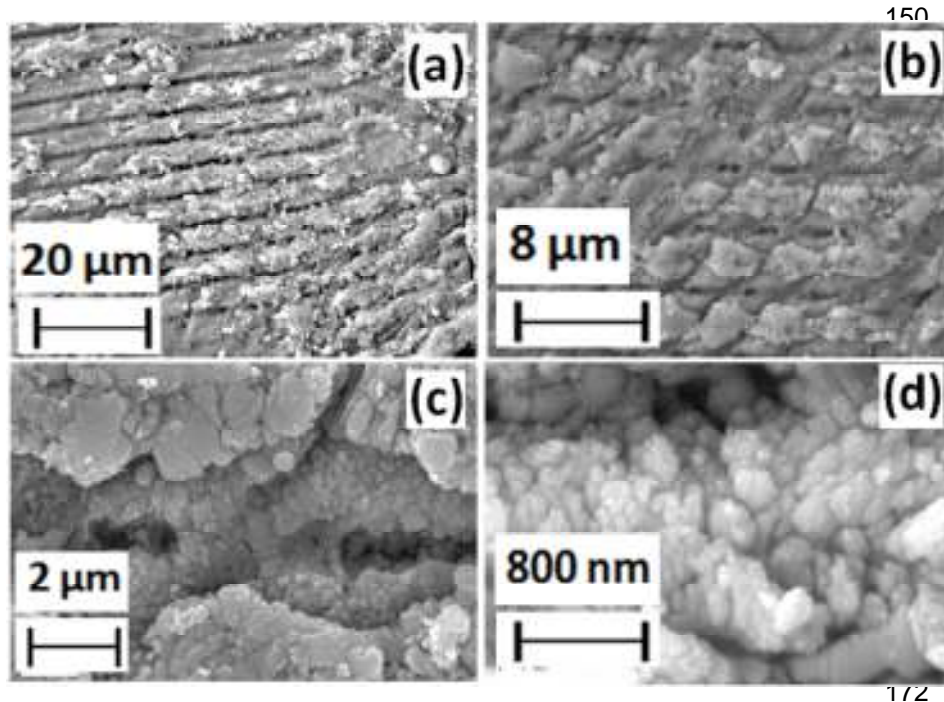
Fig. 2. Scanning electron micrographs of laser treated ZnTe thin films with increasing magnification and (a) 20 \mu\text{m} , (b) 8 \mu\text{m} , (c) 2 \mu\text{m} and (d) 800 nm scale bars.
