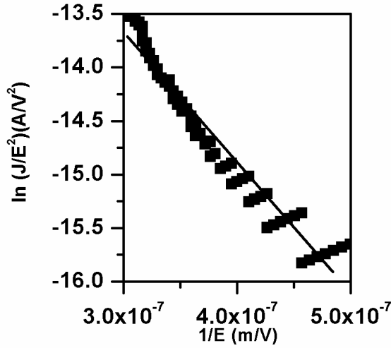
Fig. 7. The Fowler–Nordheim plots for current–voltage characteristics measured on the Au-ZnTe junction.
