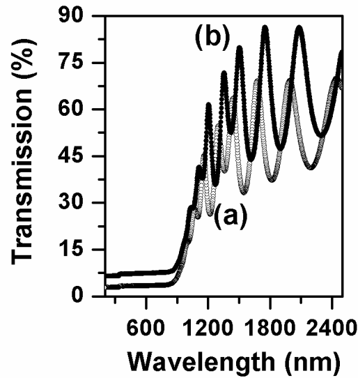
228 Fig. 3. Optical transmission spectra of (a) as deposited and (b) laser treated ZnTe thin 229 films
