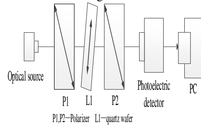
Fig.5 B The structure of the measure system
