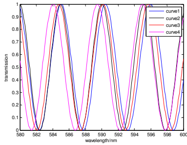
Fig.5 A The simulation results with tiny mechanical-angle at different axial directions
