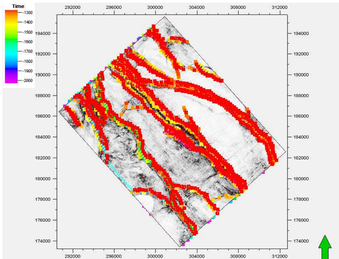
Figure 10: Variance time slice with fault sticks.
