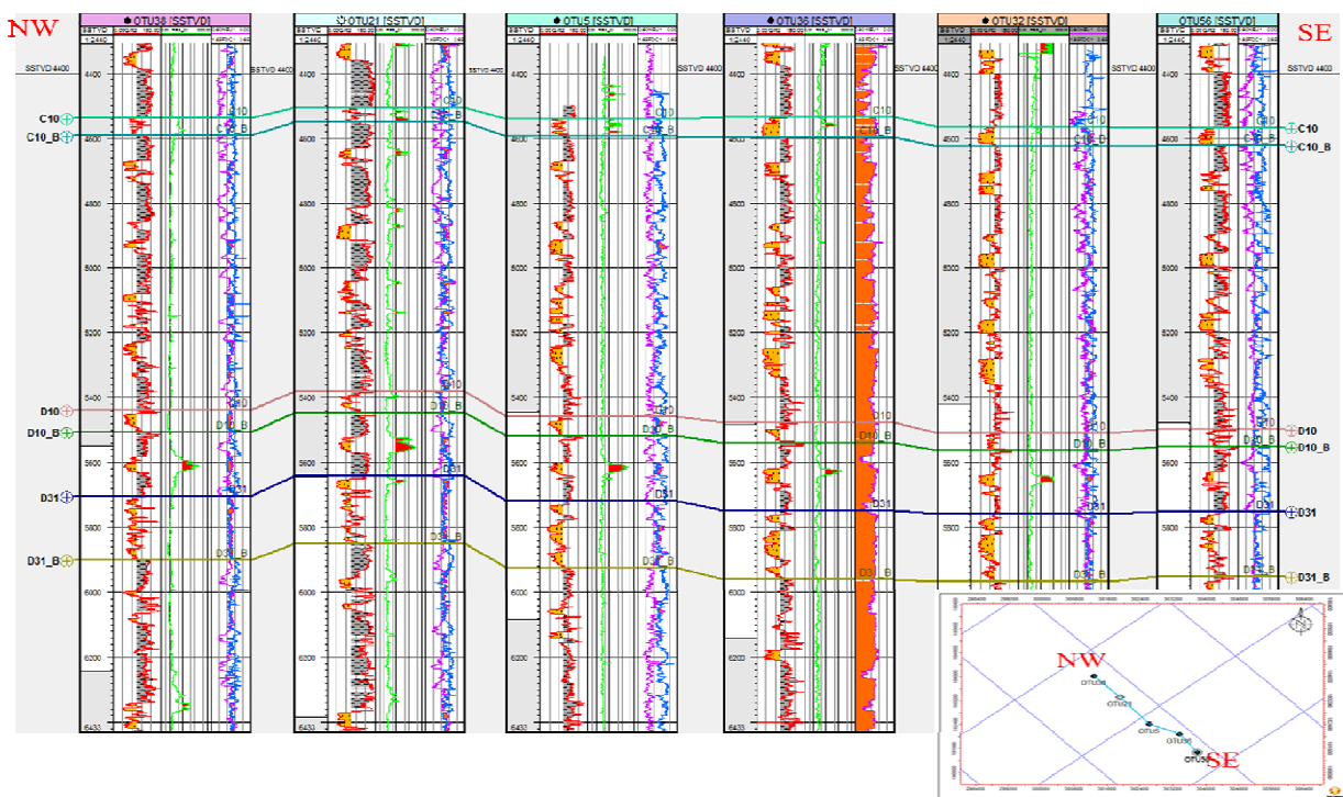
Fig. 7a: Well correlation panel of Otu Field
