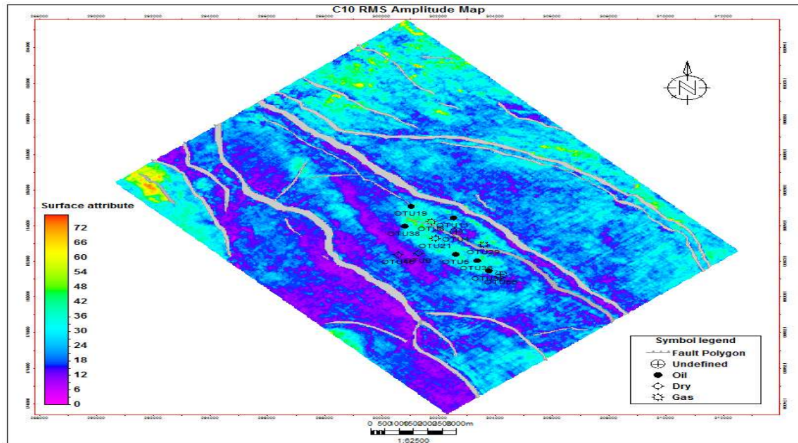
Fig. 14: RMS Amplitude for horizon C10
