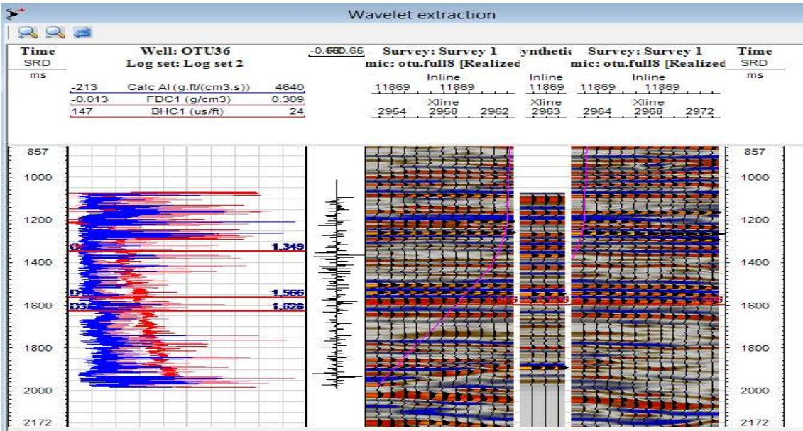
Fig. 6: Sonic calibration Otu36
