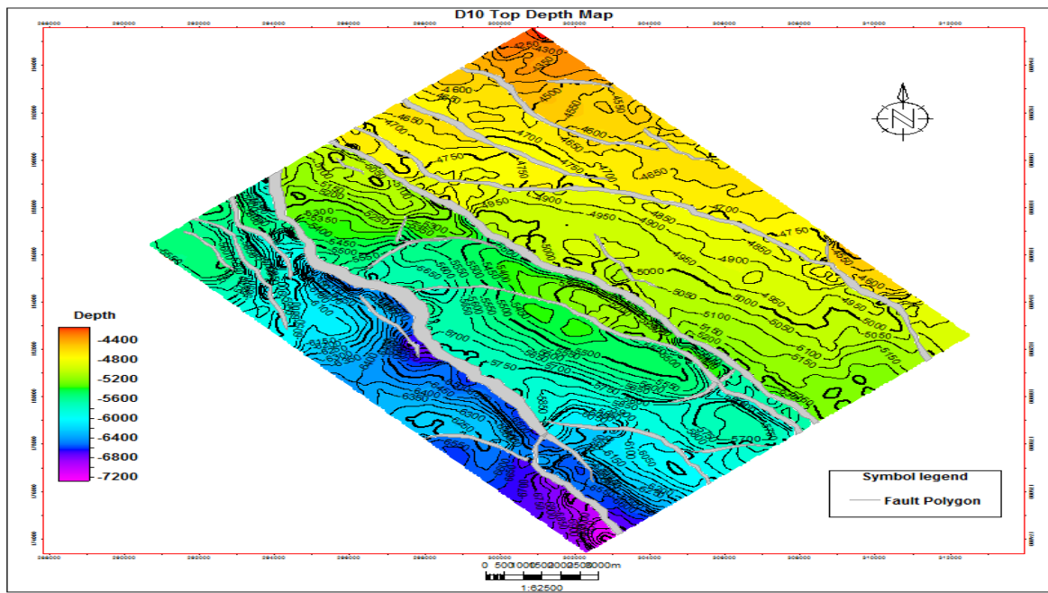
Fig. 12: Depth Structure Map of Horizon D10
